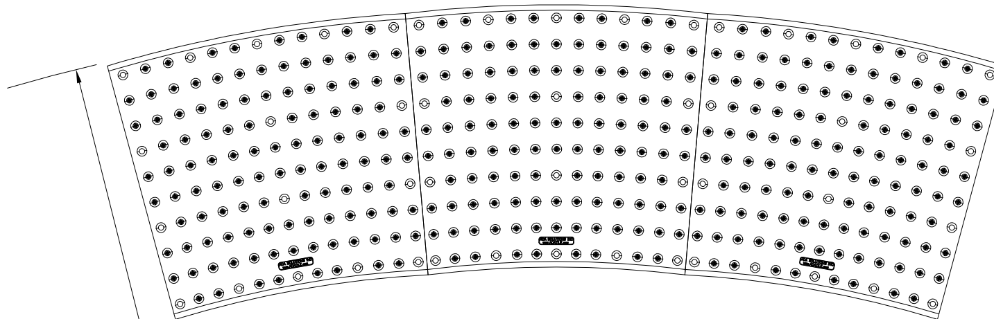
TOP VIEW OF PANEL LAYOUT IN A 15' (4.57m) RADII
